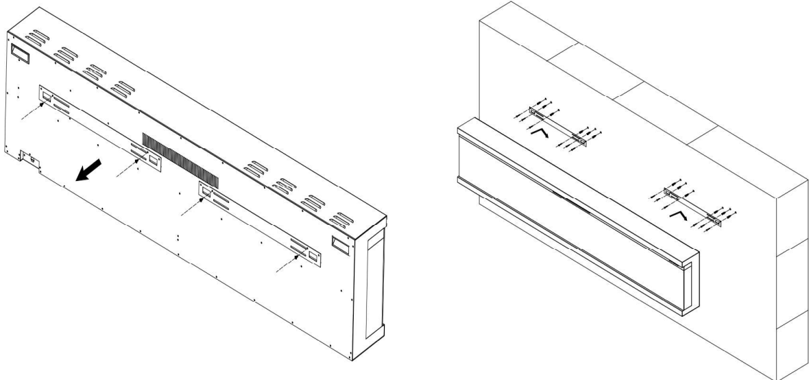
Illustration of wall bracket for model EF-NORF72
